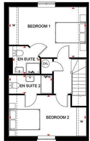
Second Floor Bedroom 1 En Suite 1 Bedroom 2 En Suite 2 (Approximate dimensions) 4990 x 3244 mm 16'4" x 10'7" 1755 x 1785 mm 5'9" x 5'10" 4990 x 2634 mm 16'4" x 8'7" 2801 x 1200 mm 9'2" x 3'11"
