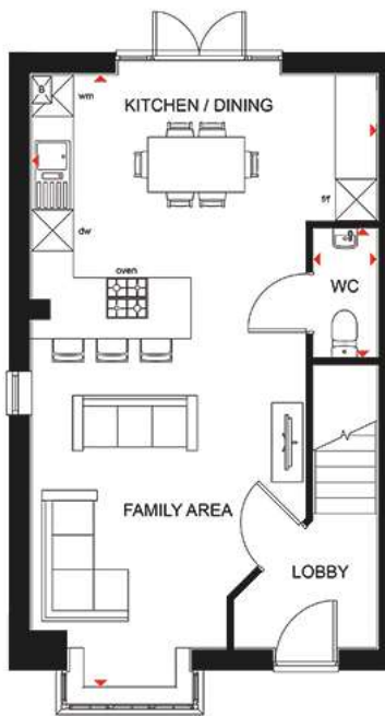
Ground Floor Kitchen/Dining/Family WC (Approximate dimensions) 4490 x 8875 mm 14'8" x 29'1" 920 x 1897 mm 3'0" x 6'2"
